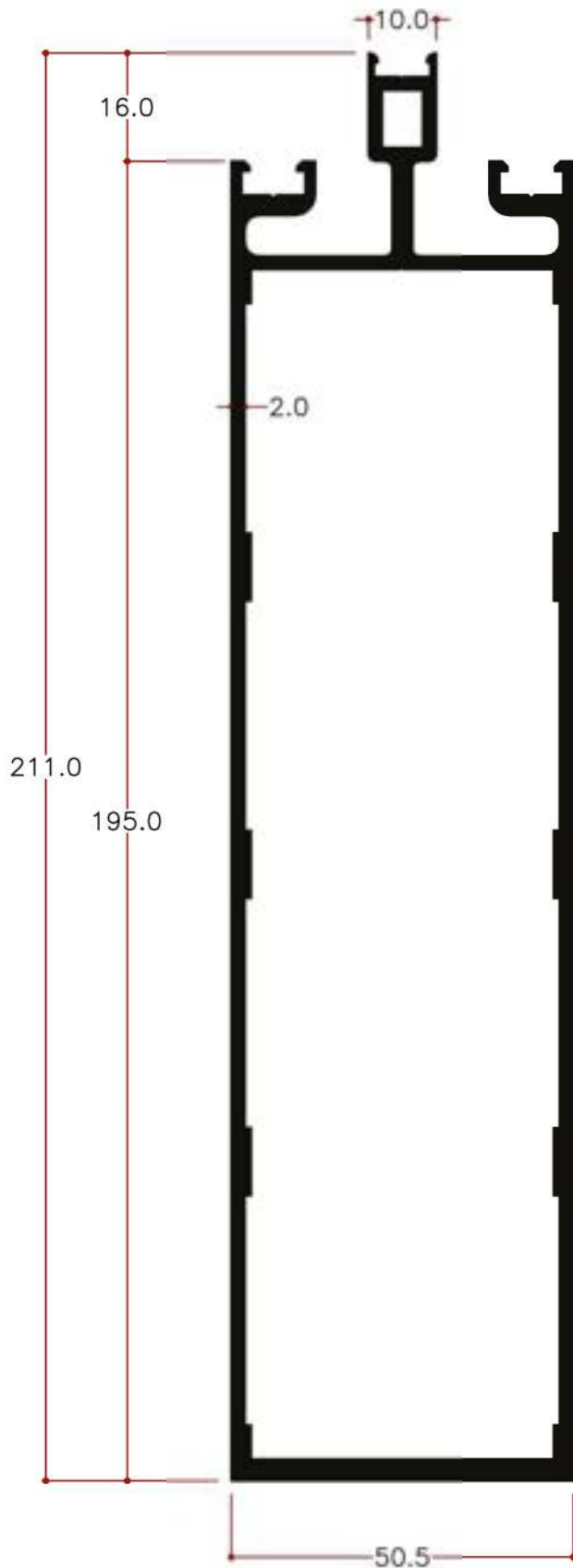
Y1807 3.494Kg/m Mullion 195 mm
