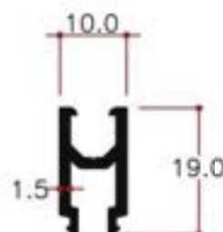
19 mm glazing adaptor This adaptor use for only S.G.50.5
