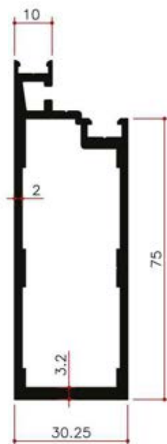
Half Transom 75 mm
