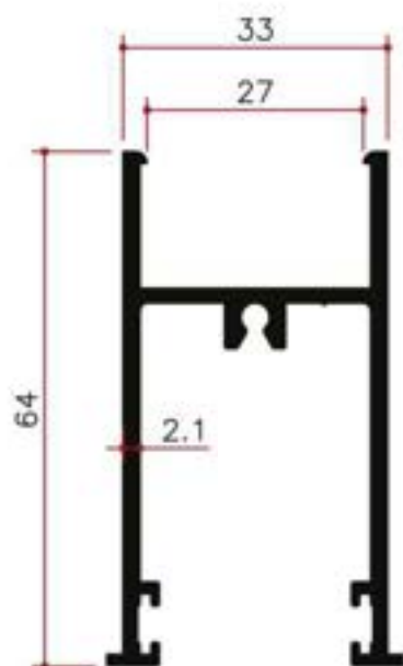
Y14718 1.005Kg/m
