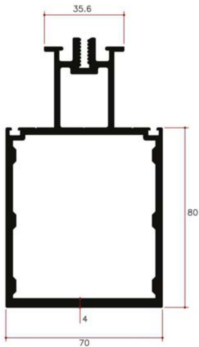
Y24940 3.573Kg/m
