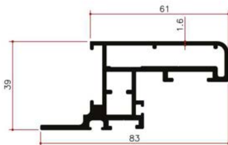
Y22624 1.387Kg/m
