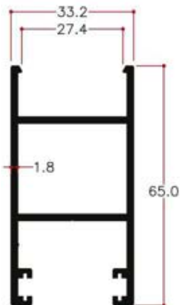
Y22469 1.015Kg/m
