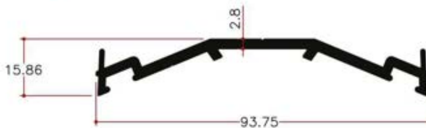
Y13608 0.893Kg/m
