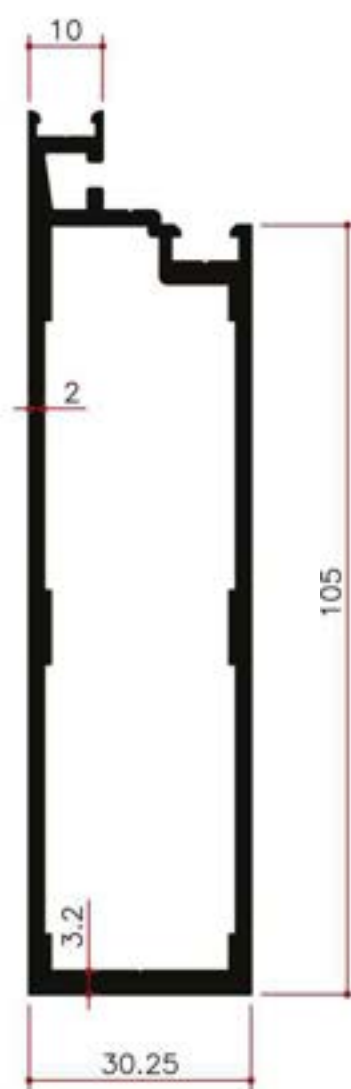
Half Transom 105 mm
