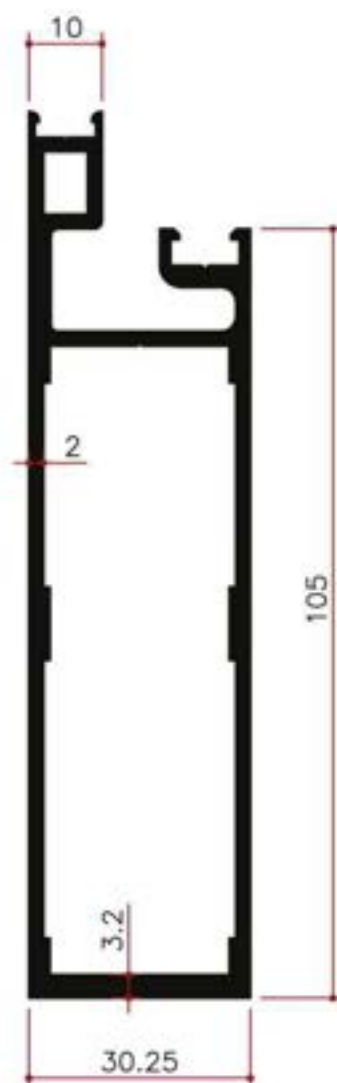
Half Mullion 105 mm
