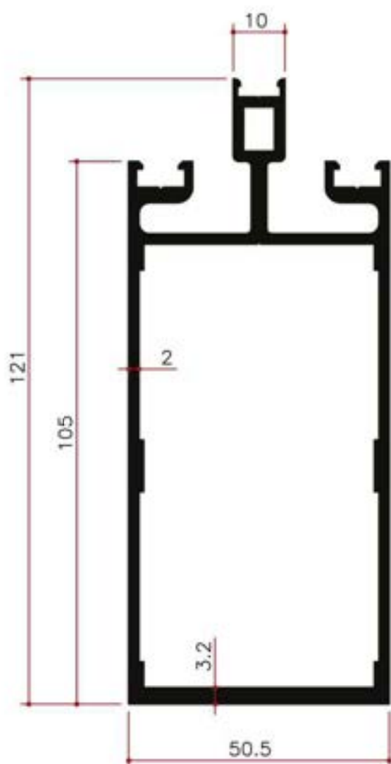
Mullion 105 mm
