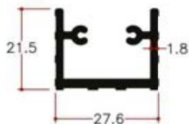
Y13536 1.823Kg/m
