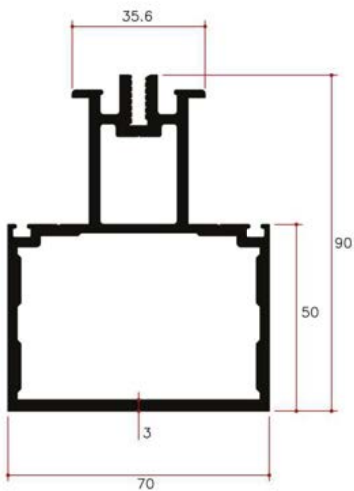
Y22389 2.772Kg/m
