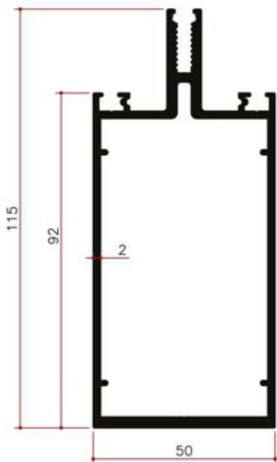
Y24364 2.082Kg/m
