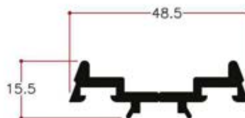
Pressure plate
