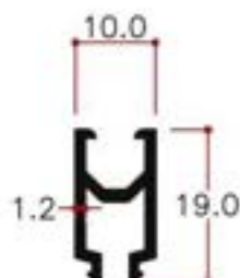
19 mm glazing adaptor This adaptor use for only S.G.50
