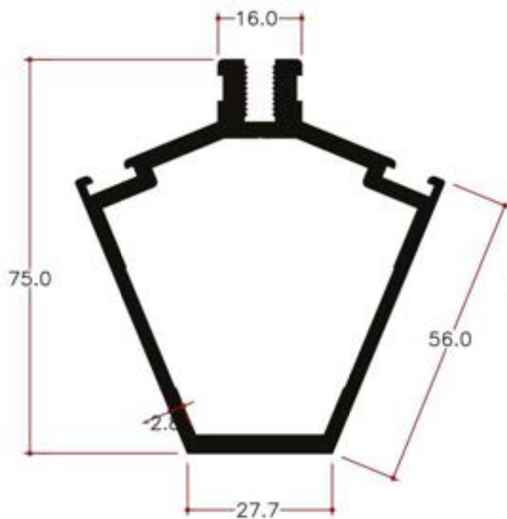
Y23684 1.979Kg/m
