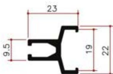
D/G spacer 2 sided structural
