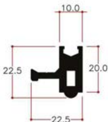
20mm Clamp block structural
