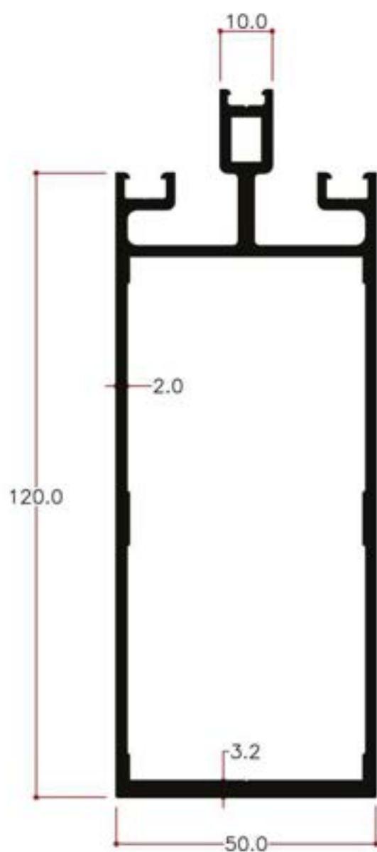
Mullion 120 mm
