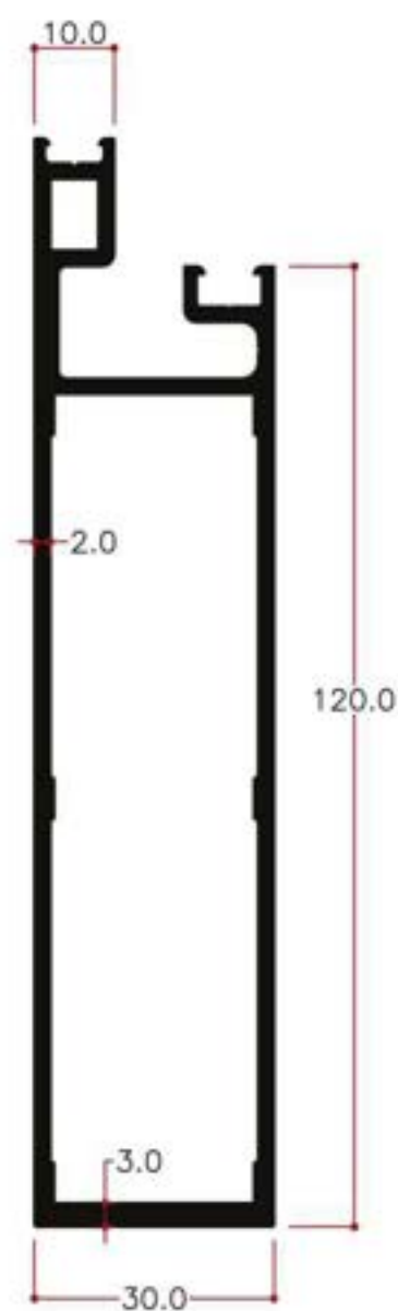
Half Mullion 120 mm
