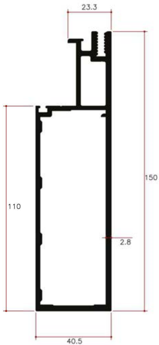
Y21626 2.845Kg/m
