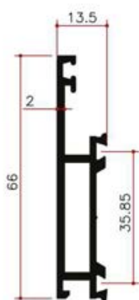
Y22257 0.737Kg/m
