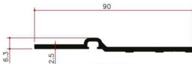
Y12431 0.652Kg/m
