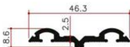
Y13984 0.319Kg/m
