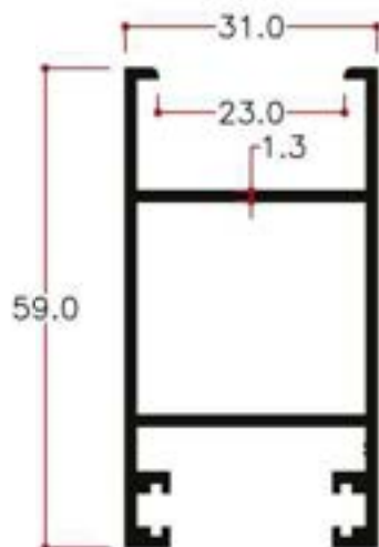
Y21650 0.722Kg/m
