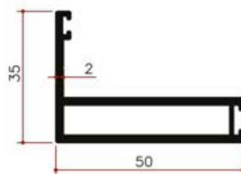
Y24367 0.754Kg/m
