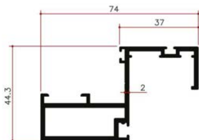
Y24803 1.150Kg/m
