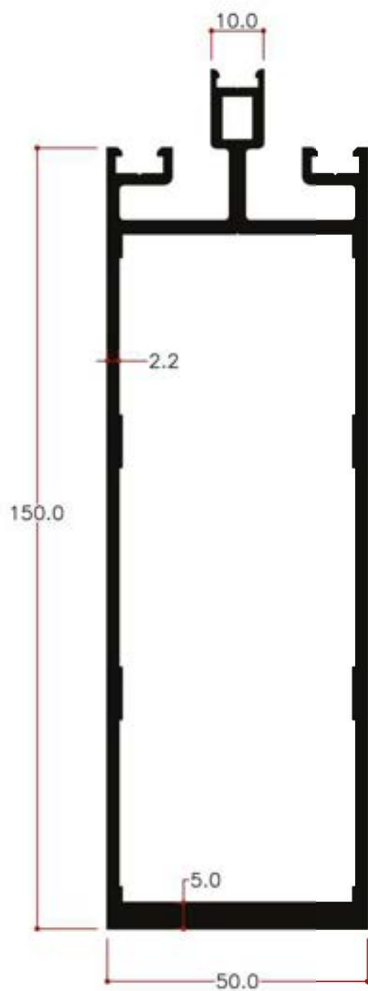
Mullion 150 mm
