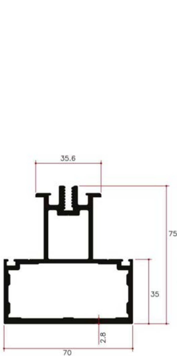
Y22623 2.298Kg/m
