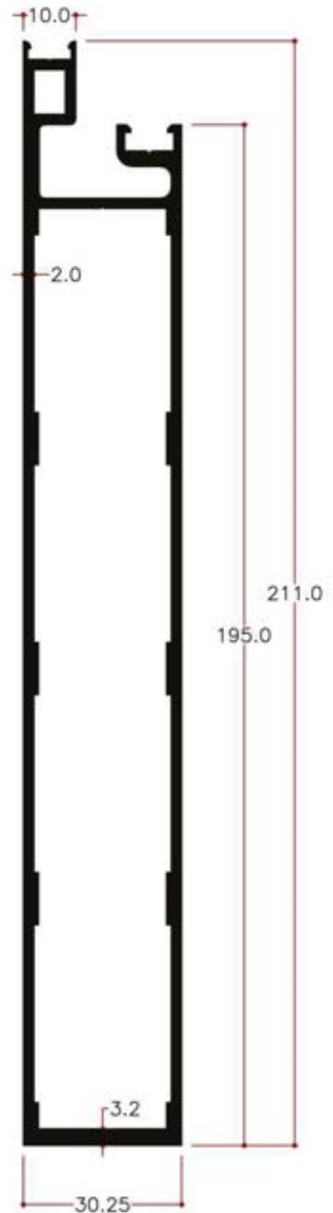
Y26031 3.029Kg/m Half Mullion 195 mm
