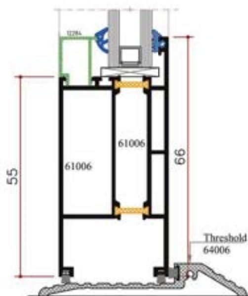
DETAIL - E
