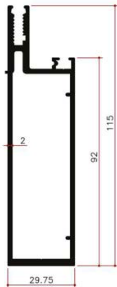
Y24699 1.735Kg/m
