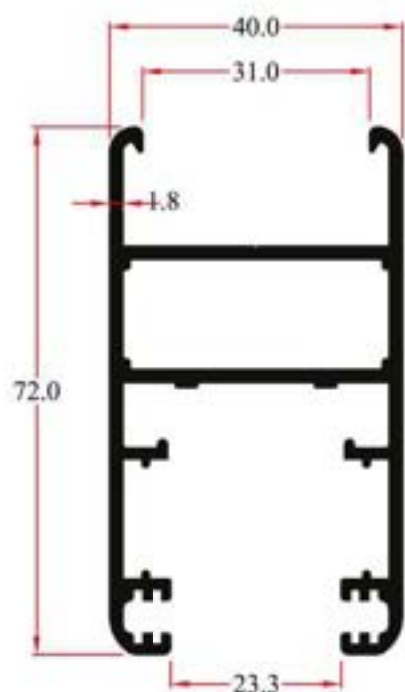
Y26210 1.305Kg/m
