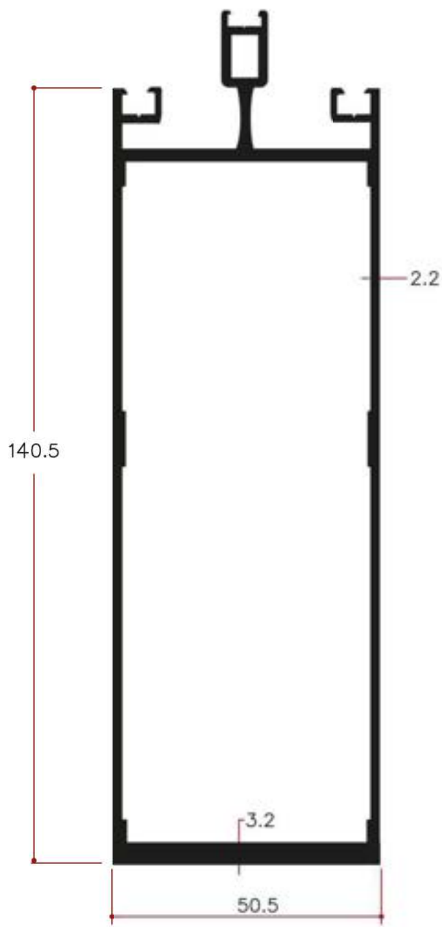
Y1805 3.031 Kg/m
