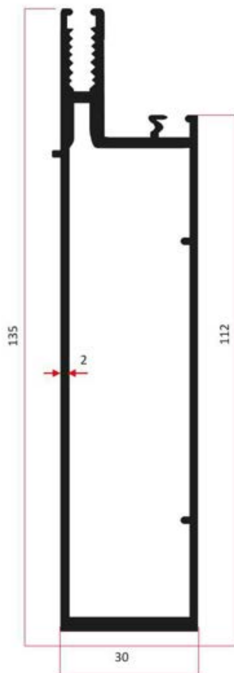
Y29629 1.951 Kg/m
