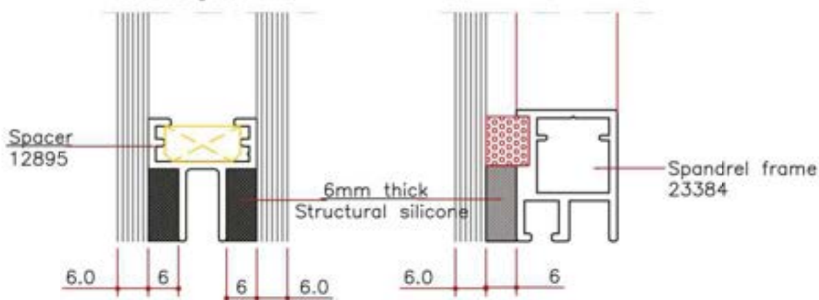
Double glass unit
