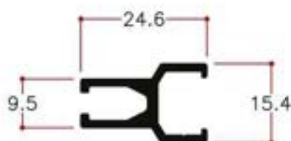
D/G spacer 2 sided structural
