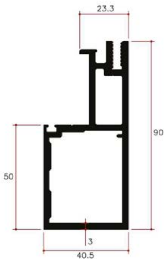
Y22390 2.190Kg/m
