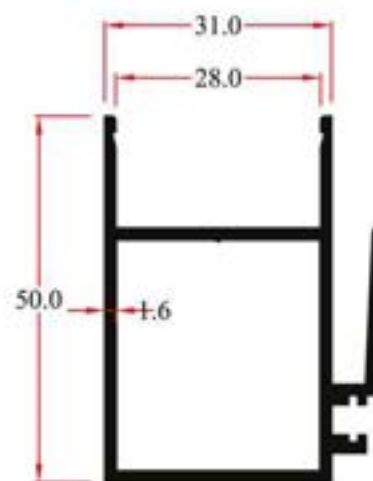
Y25315 0.822Kg/m
