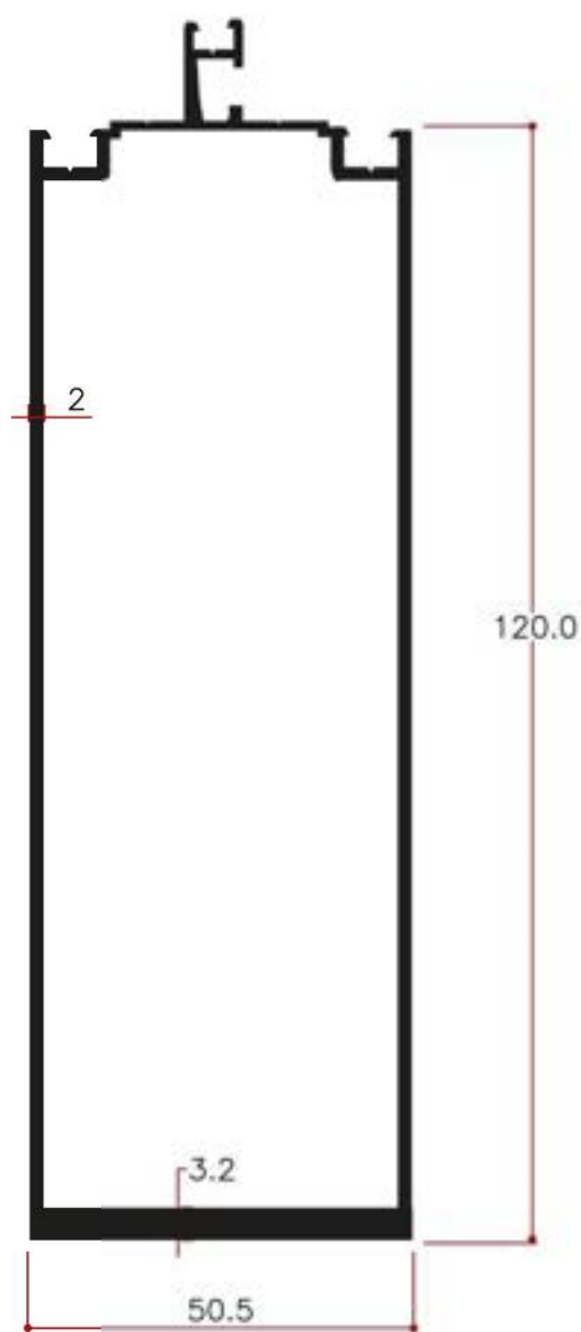
Y5980 2.173 Kg/m
