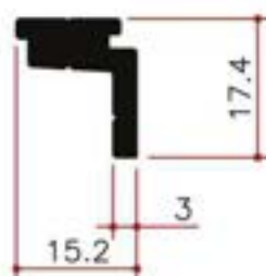
Y12430 0.301Kg/m
