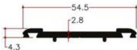
Y13605 0.428Kg/m
