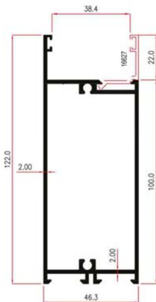
Y24952 1.743 Kg/m
