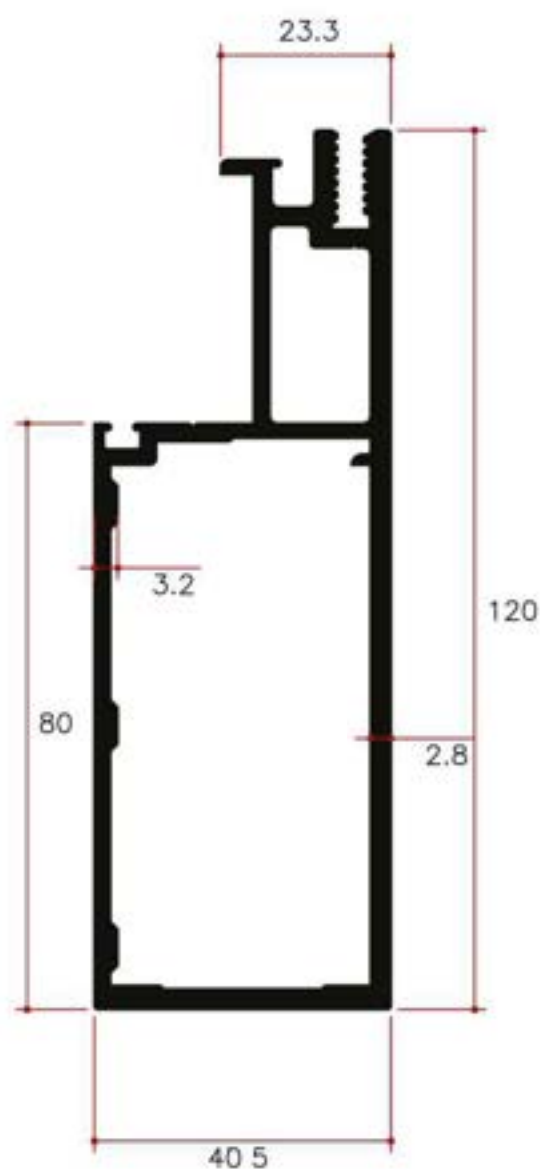
Y21624 2.423Kg/m
