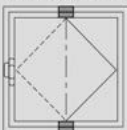
Vertical pivot-hinged sash
