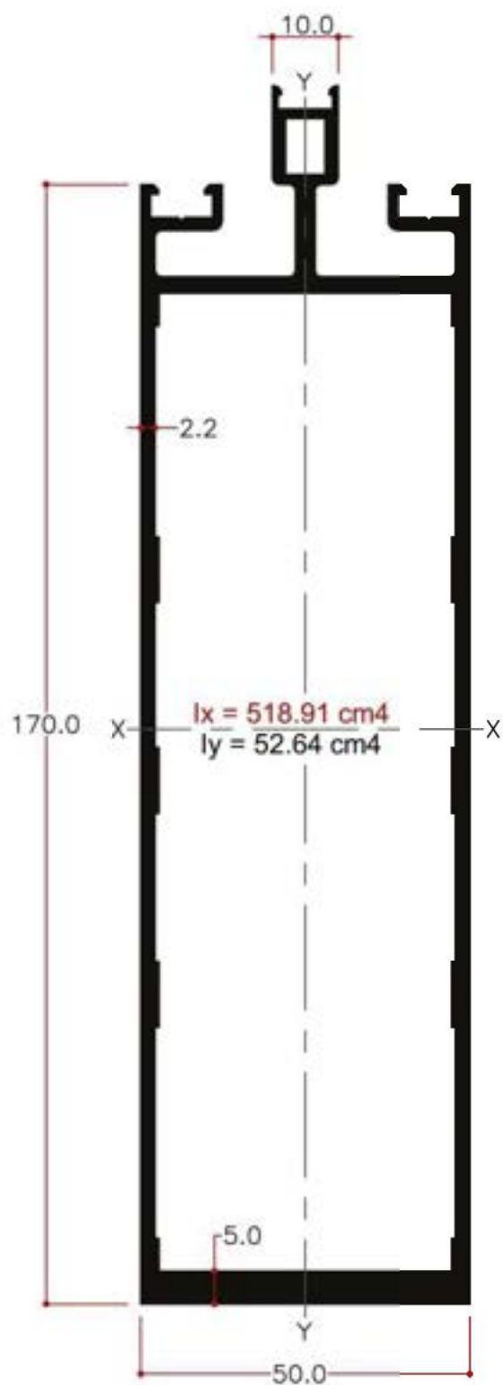
Mullion 170 mm
