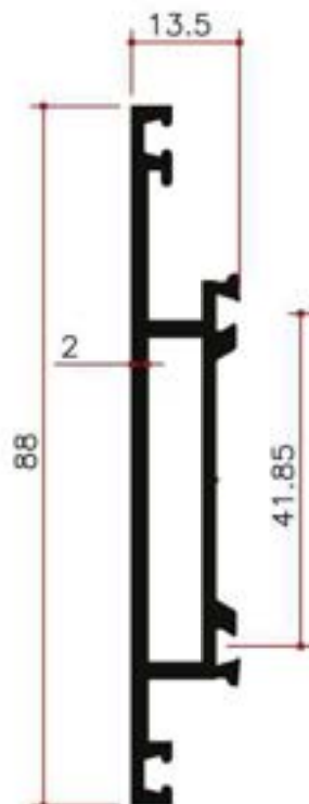
Y22260 0.907Kg/m
