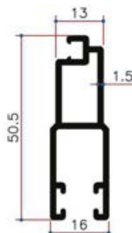
Y21440 0.565Kg/m
