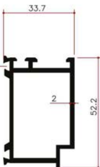
Y22261 0.927Kg/m
