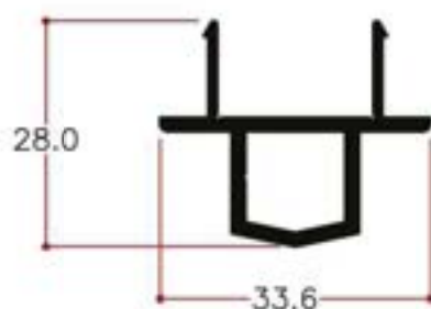
Y24058 0.399Kg/m
