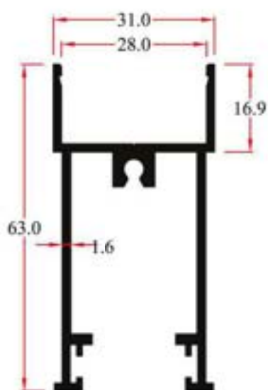
Y15118 0.838Kg/m
