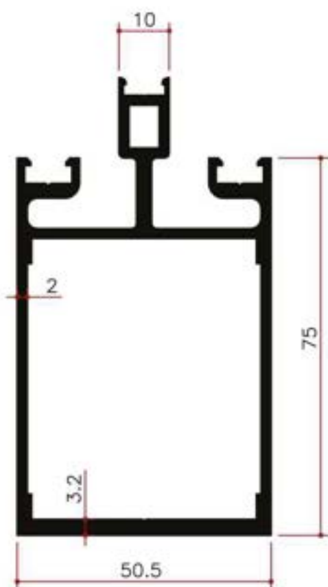
Mullion 75 mm
