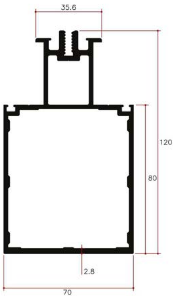
Y21623 2.895Kg/m
