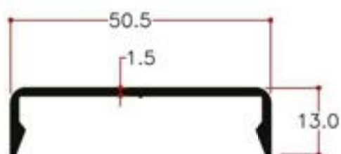
Cover cap 12.5 mm for transoms
