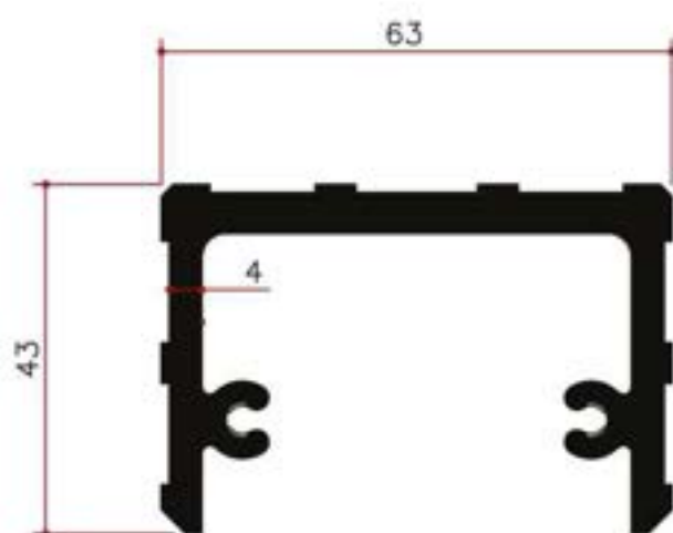
Y11577 2.038Kg/m
