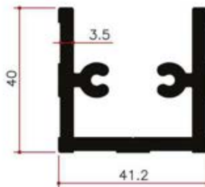
Y13986 1.431Kg/m
