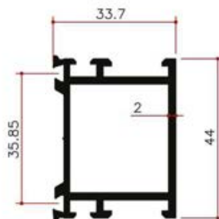
Y22258 0.914Kg/m
