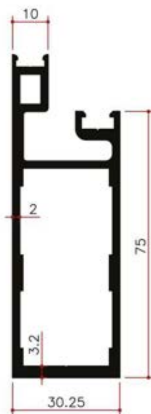
Half Mullion 75 mm
