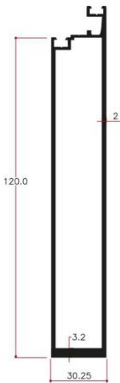
Y5981 1.941 Kg/m
