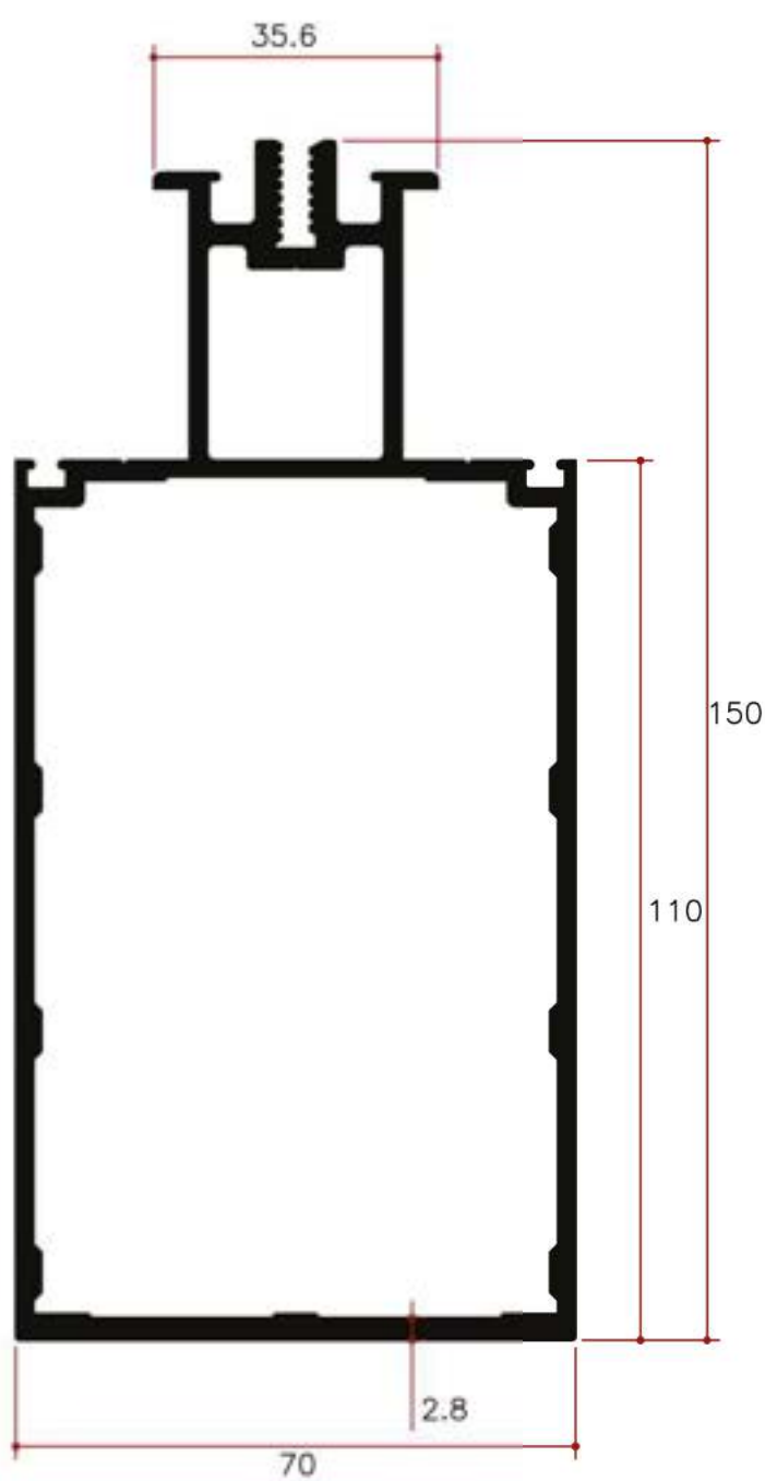
Y21625 3.254Kg/m
