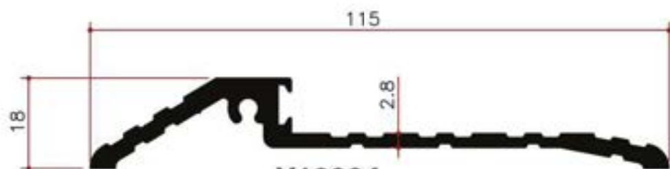
Y12324 1.127Kg/m
