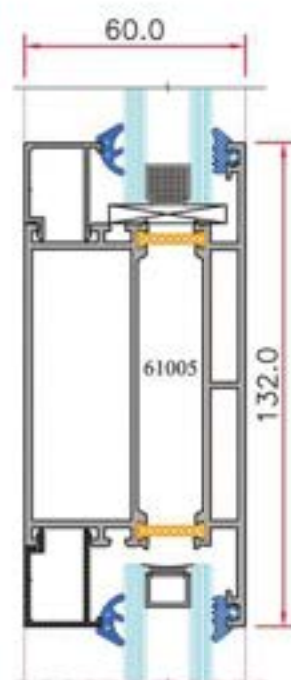
DETAIL - D
