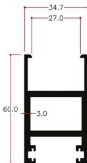
Y24726 1.335Kg/m
