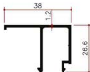
Y12368 0.328Kg/m
