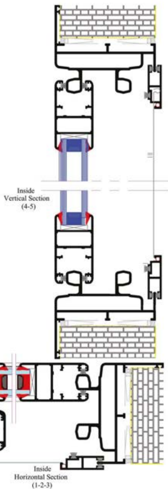
2 Panel Sliding Window Frame 24mm Double Glass With Fly Screen Outside
