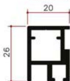
Spandrel profile for 2 sided structural
