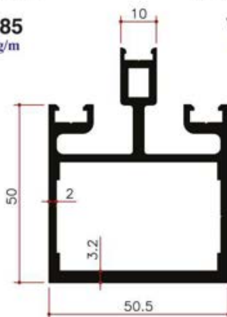
Mullion 50 mm
