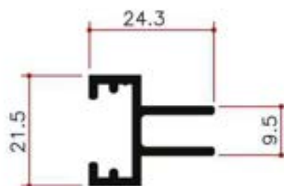
D/G spacer 4 sided structural
