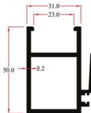
Y23963 1.095Kg/m
