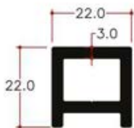
Y23461 0.613Kg/m
