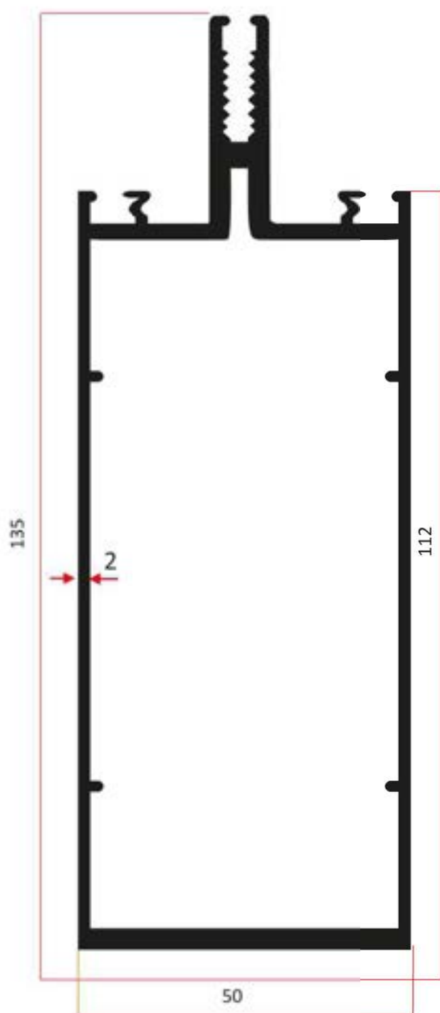
Y29227 2.310 Kg/m
