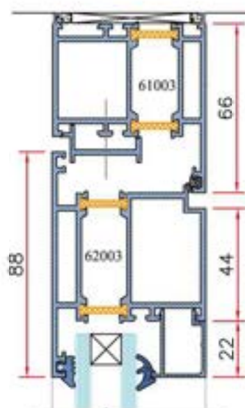
DETAIL - C
